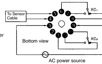
61F-GPN-V50 Water Leak Detector
